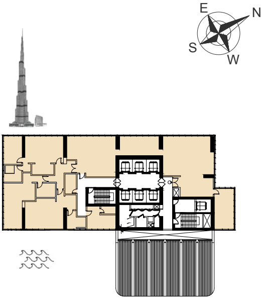
T9- FLOOR: 48
