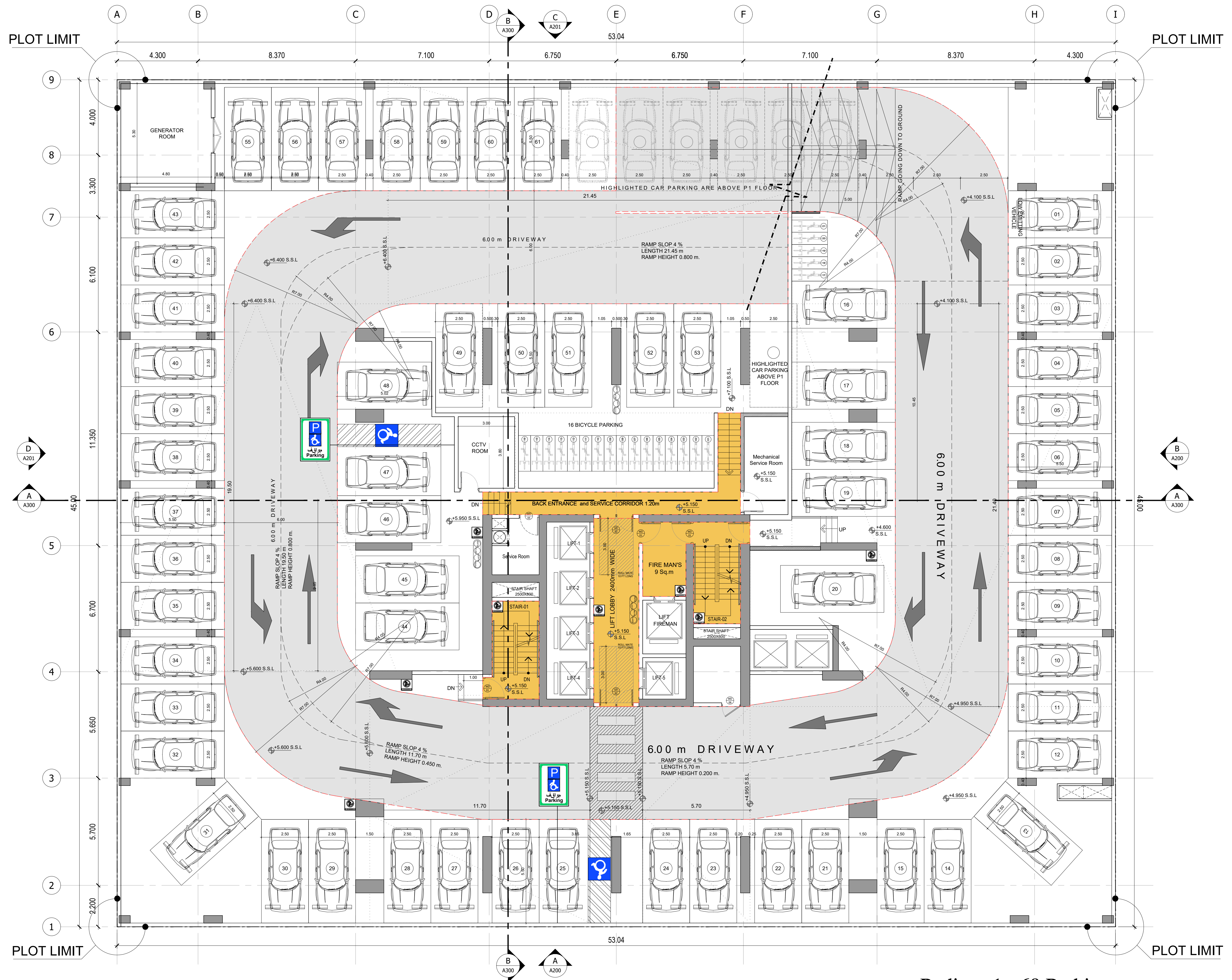
Podium-1 - 60 Parking
