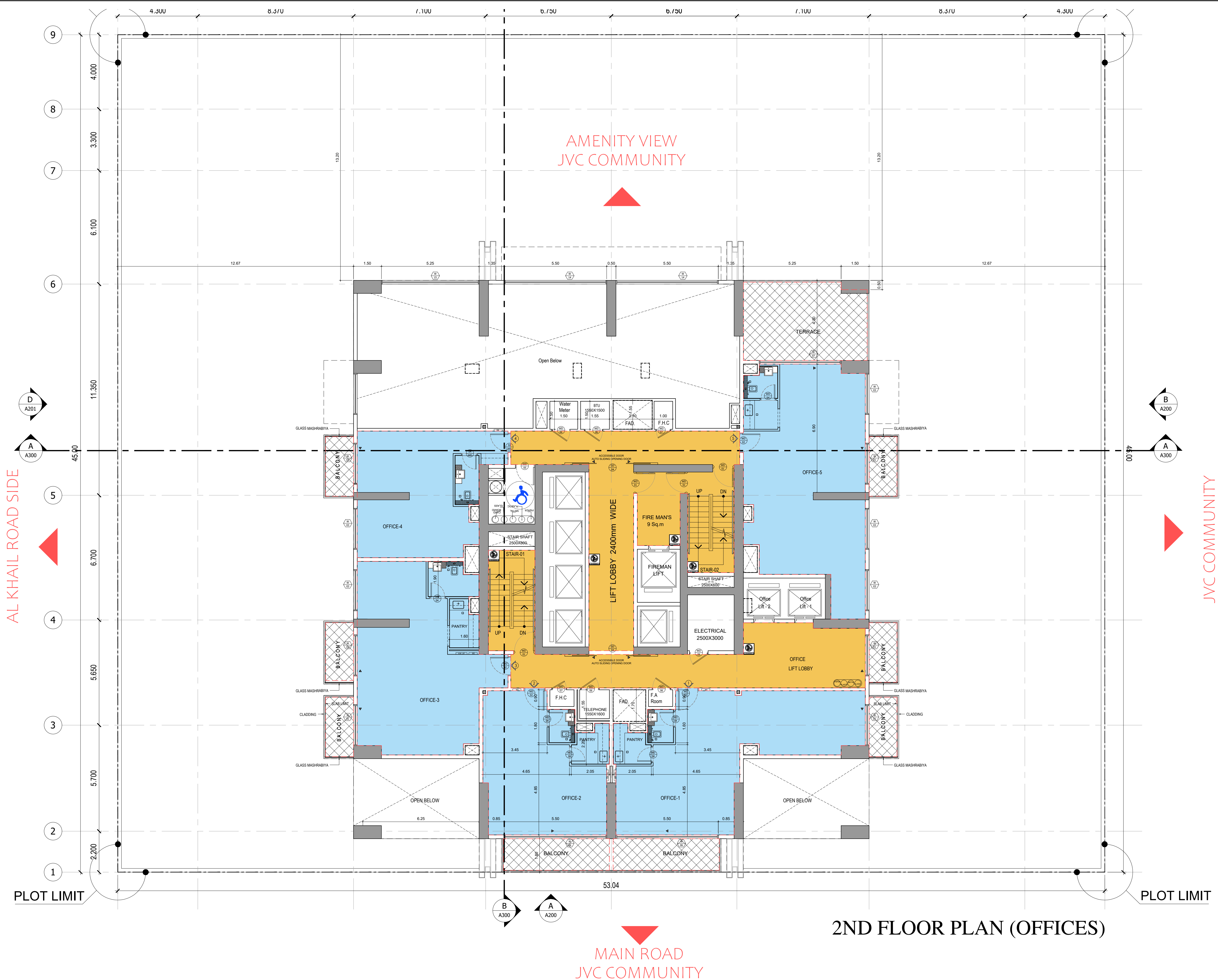
2ND FLOOR PLAN (OFFICES)
