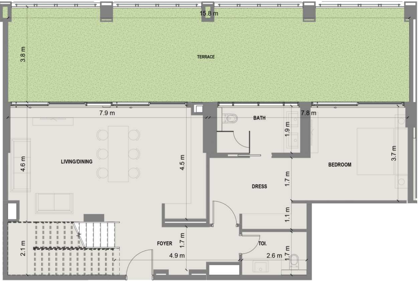
GROUND FLOOR
