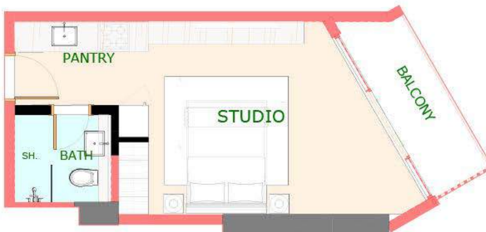
APARTMENT LAYOUT
