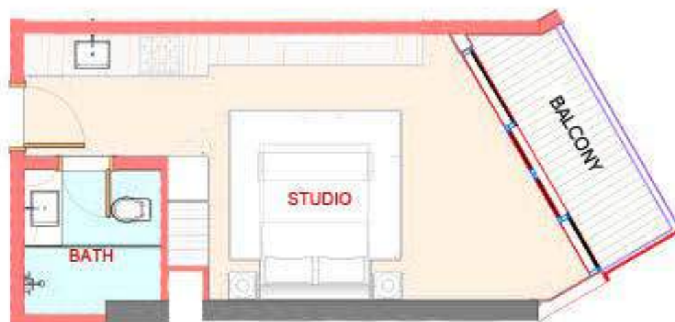
APARTMENT LAYOUT
