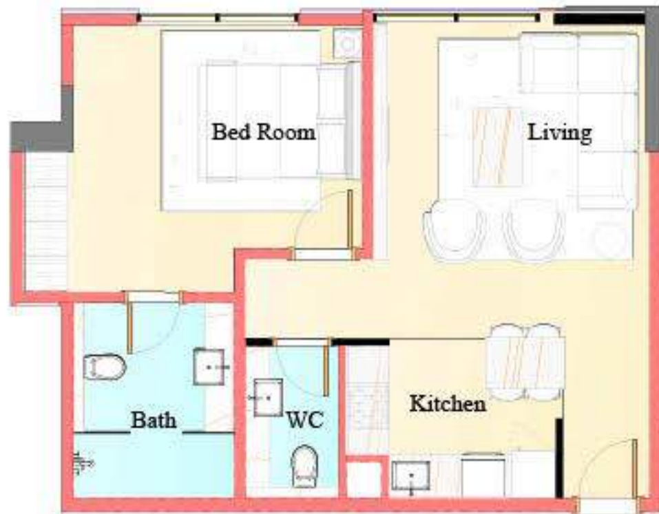
APARTMENT LAYOUT
