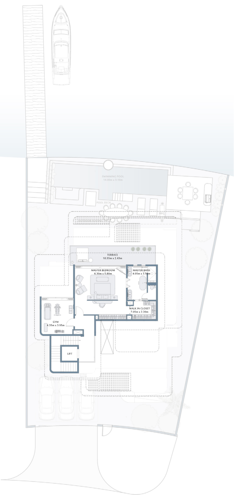
SECOND FLOOR
