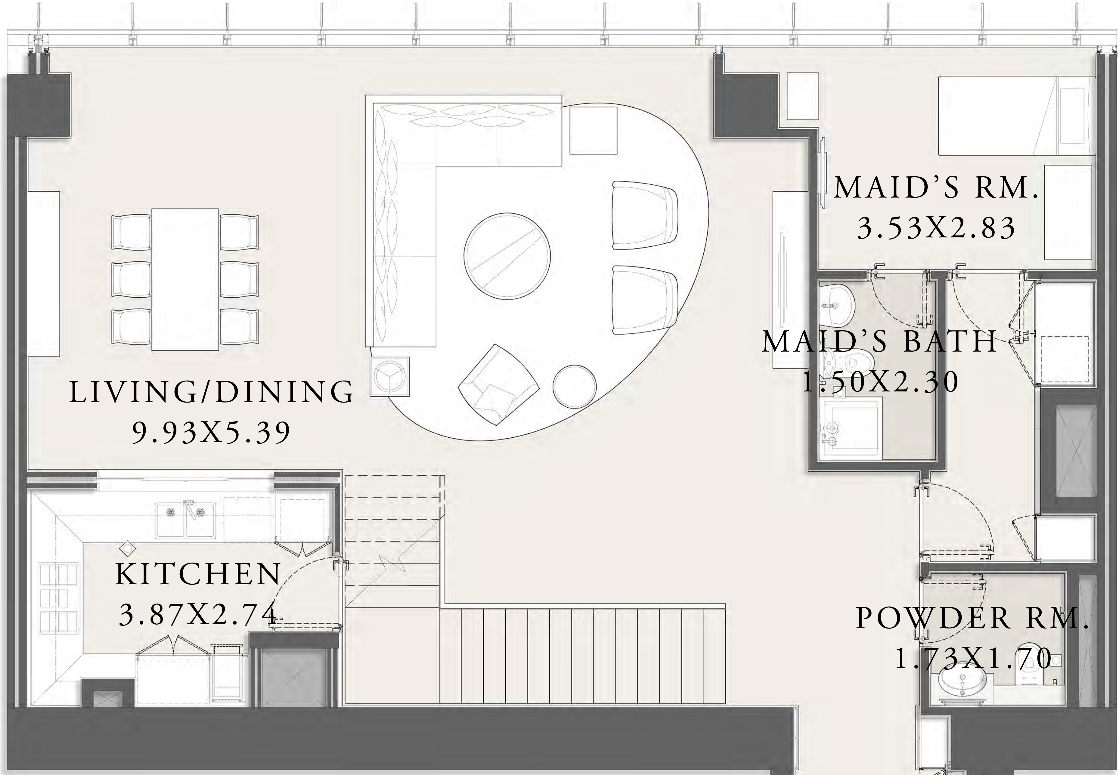
LOWER LEVEL
