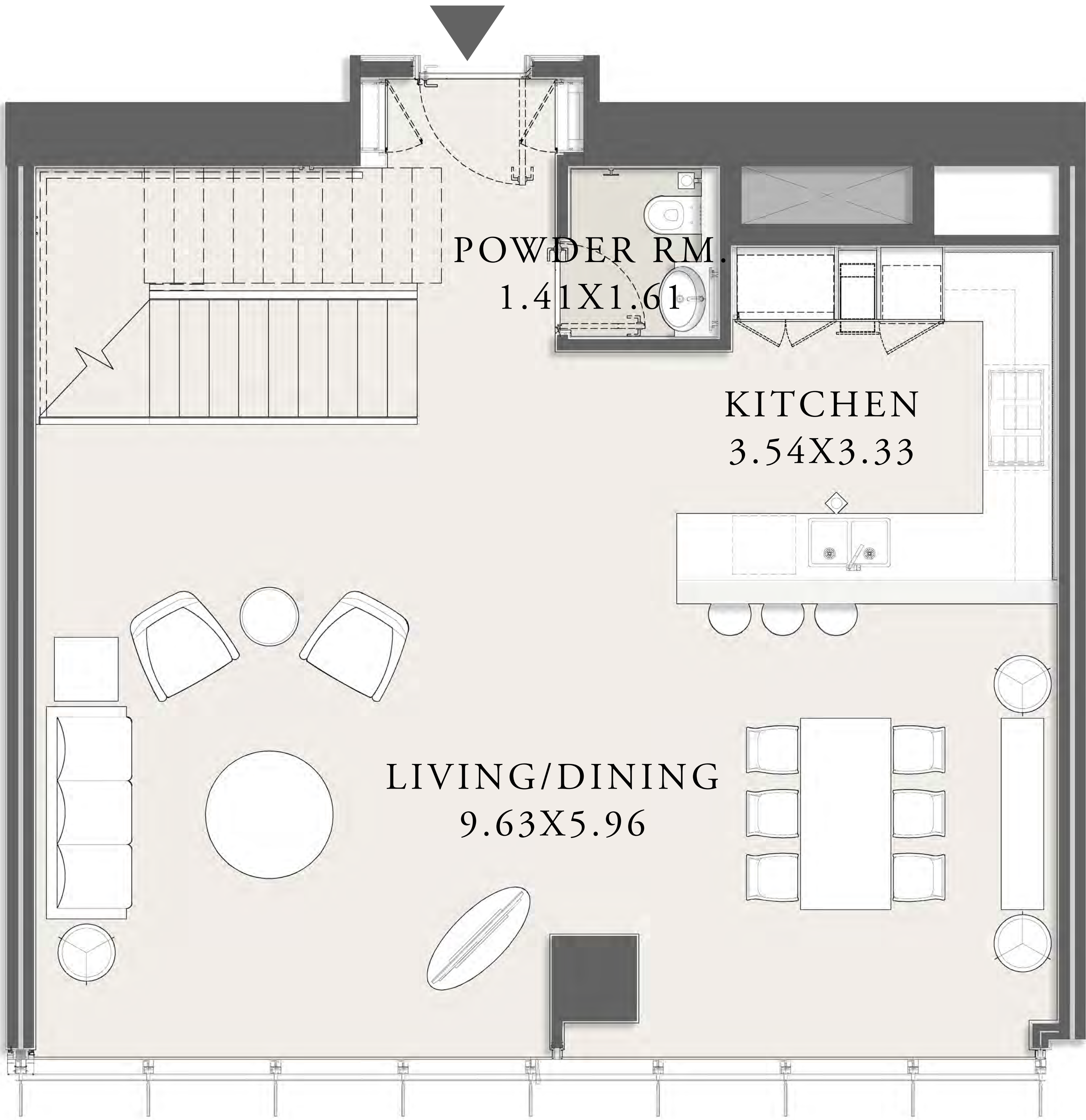
LOWER LEVEL
