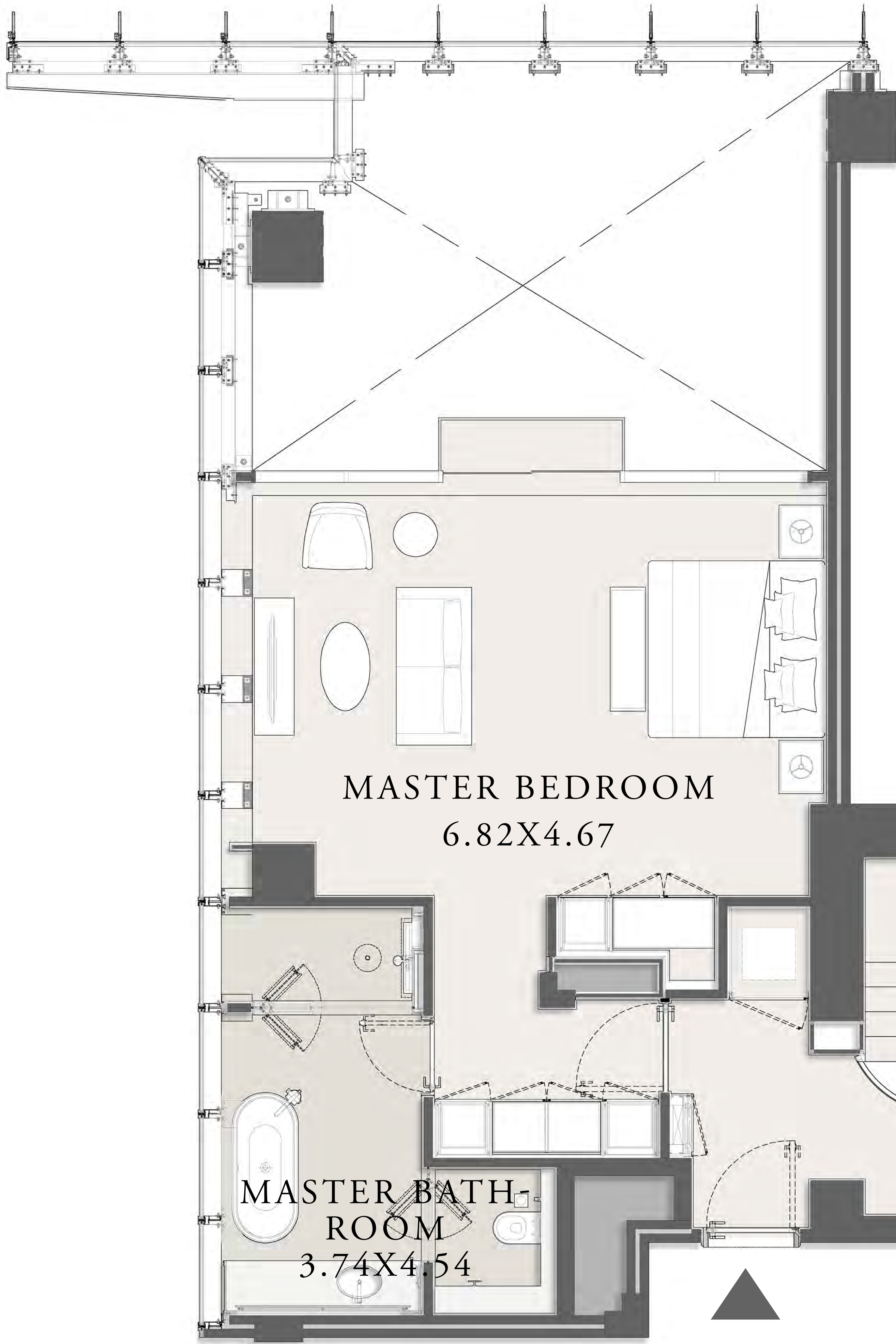
UPPER LEVEL
