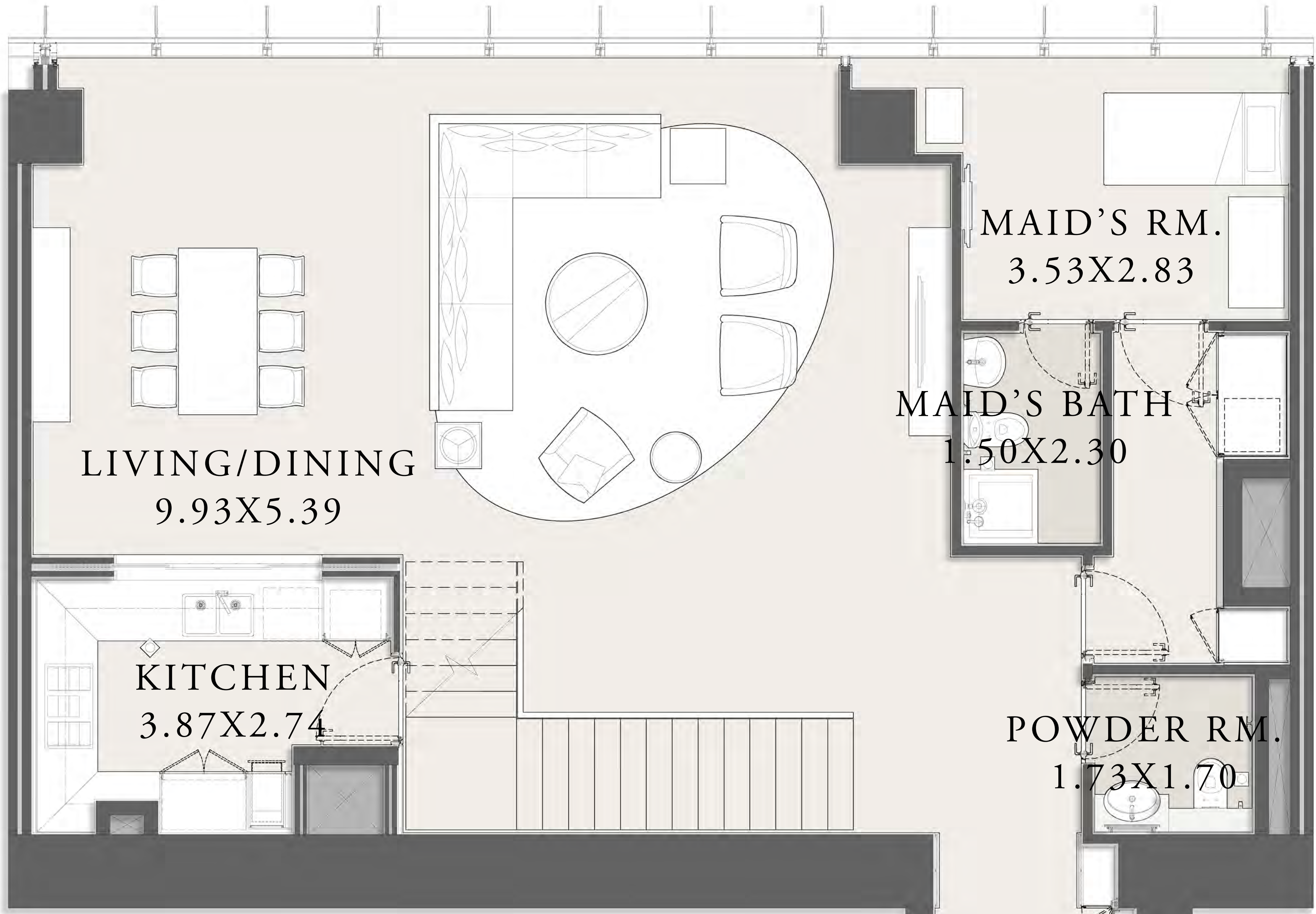
LOWER LEVEL
