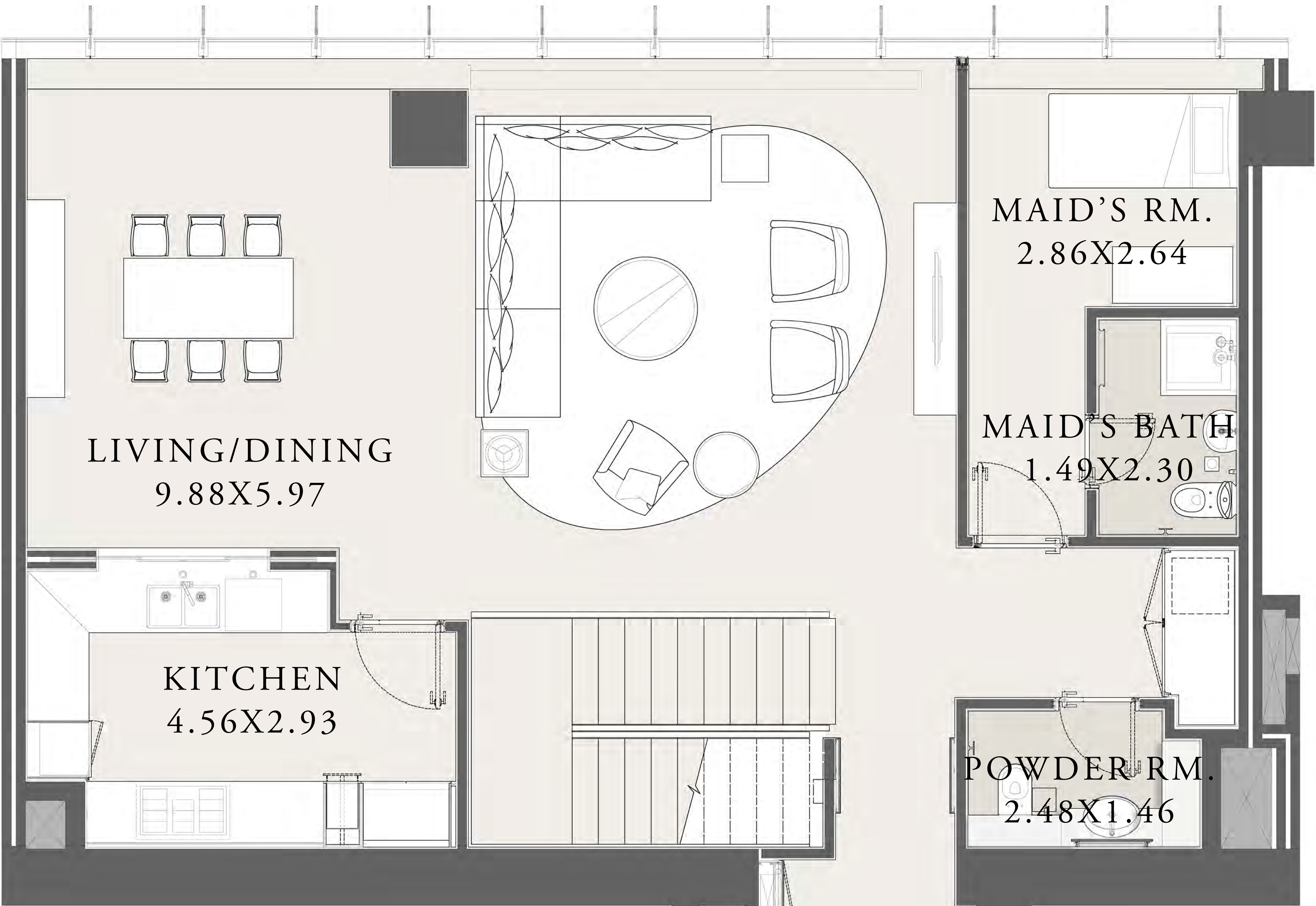
LOWER LEVEL
