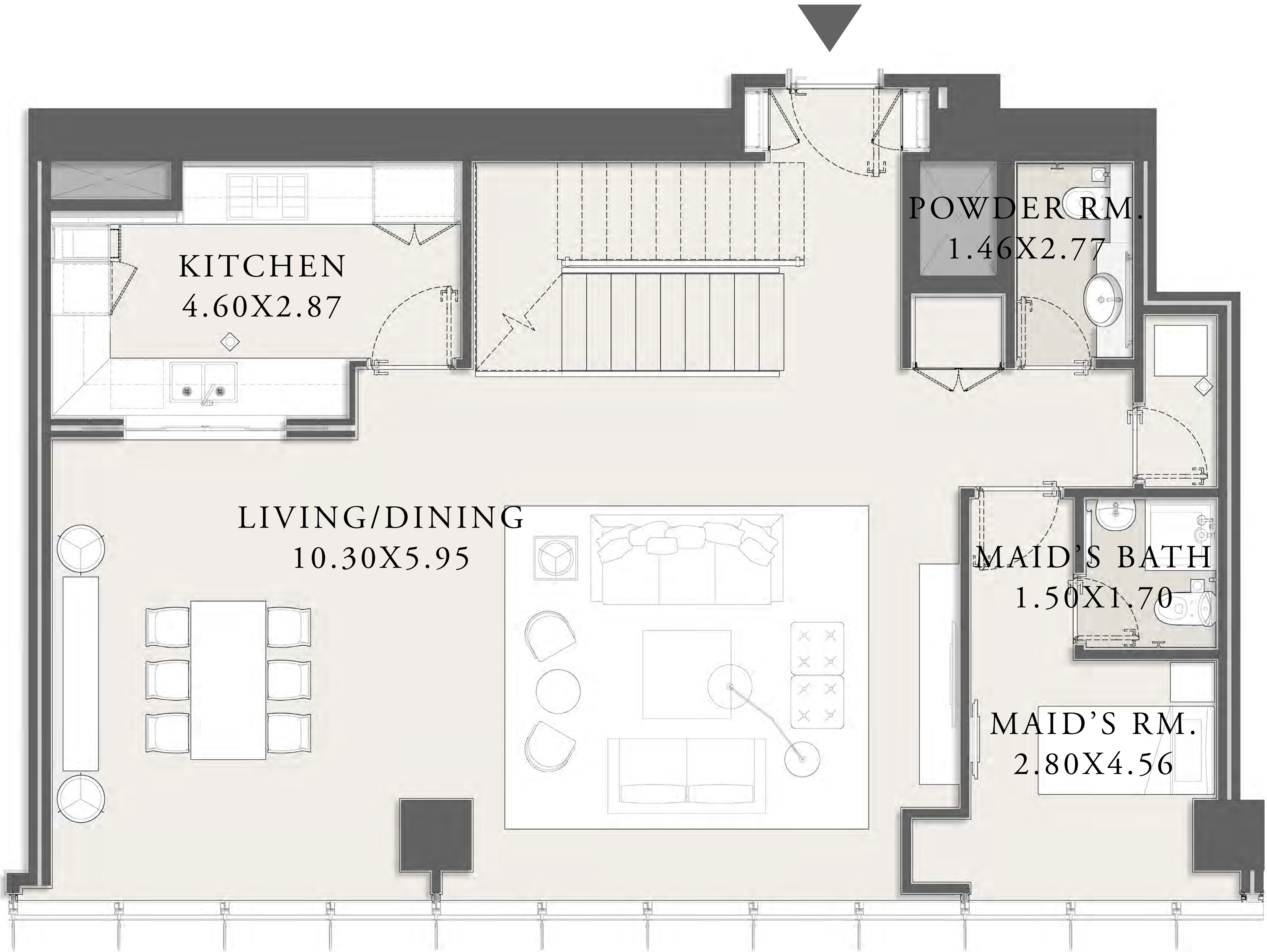
LOWER LEVEL
