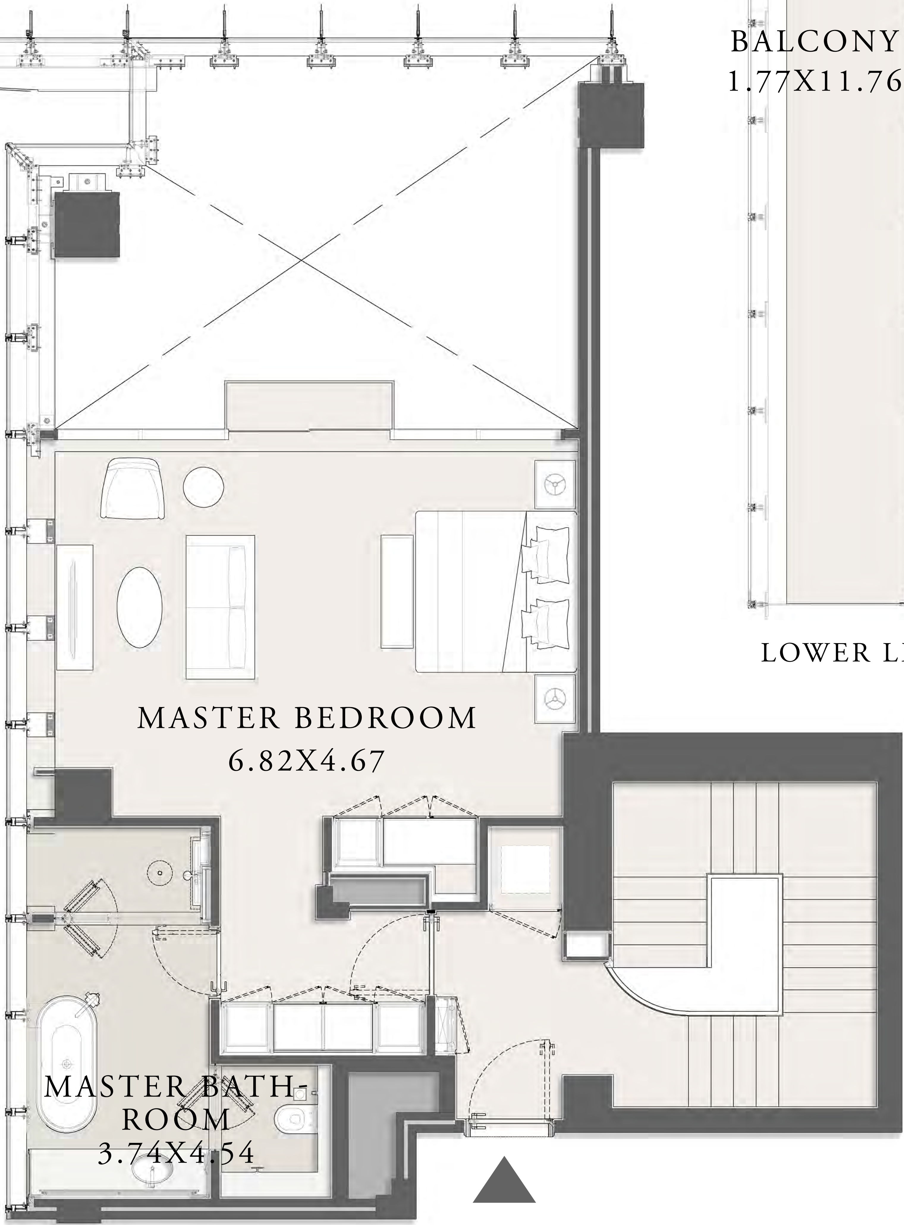
UPPER LEVEL
