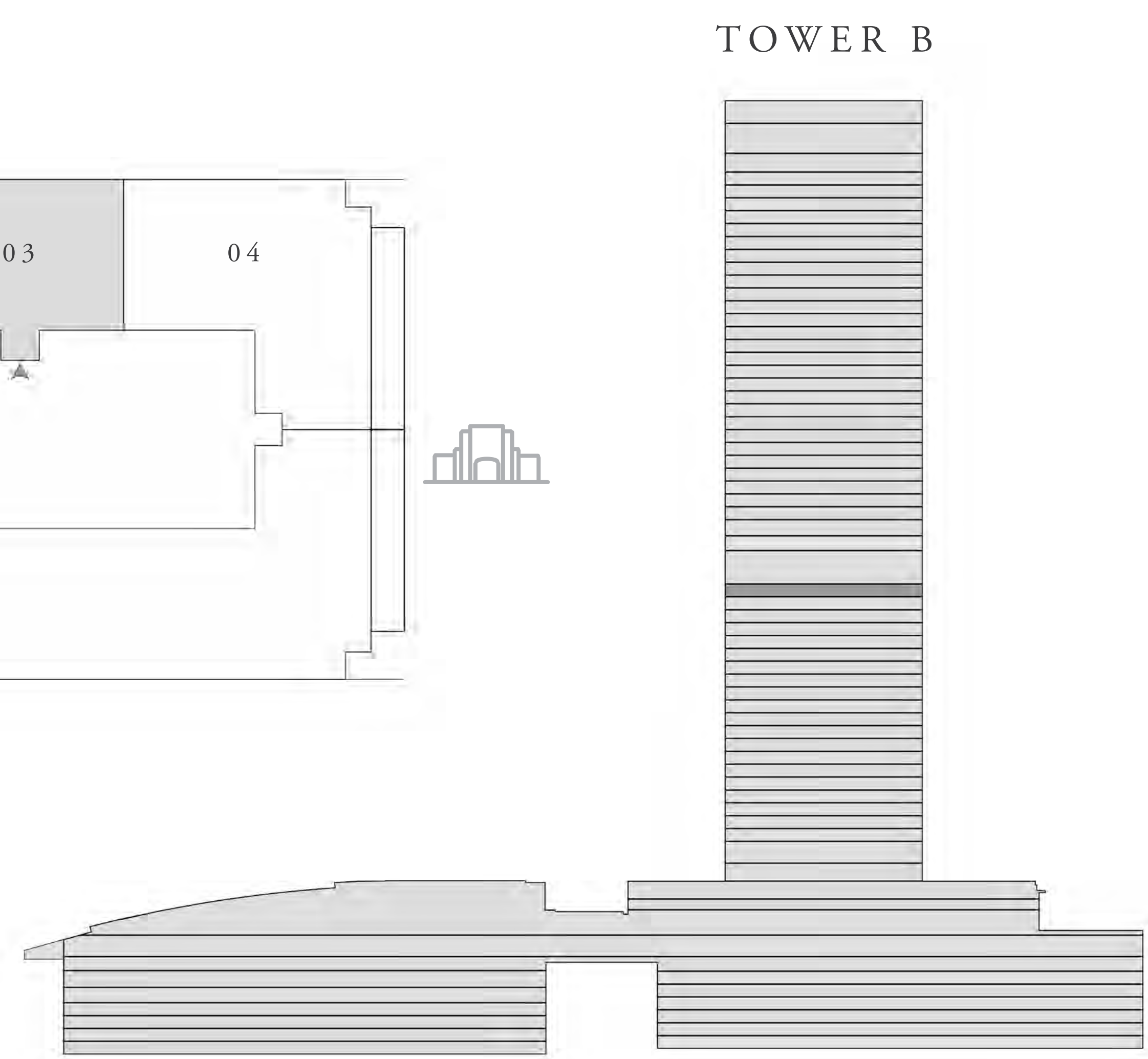
KEY SECTION
