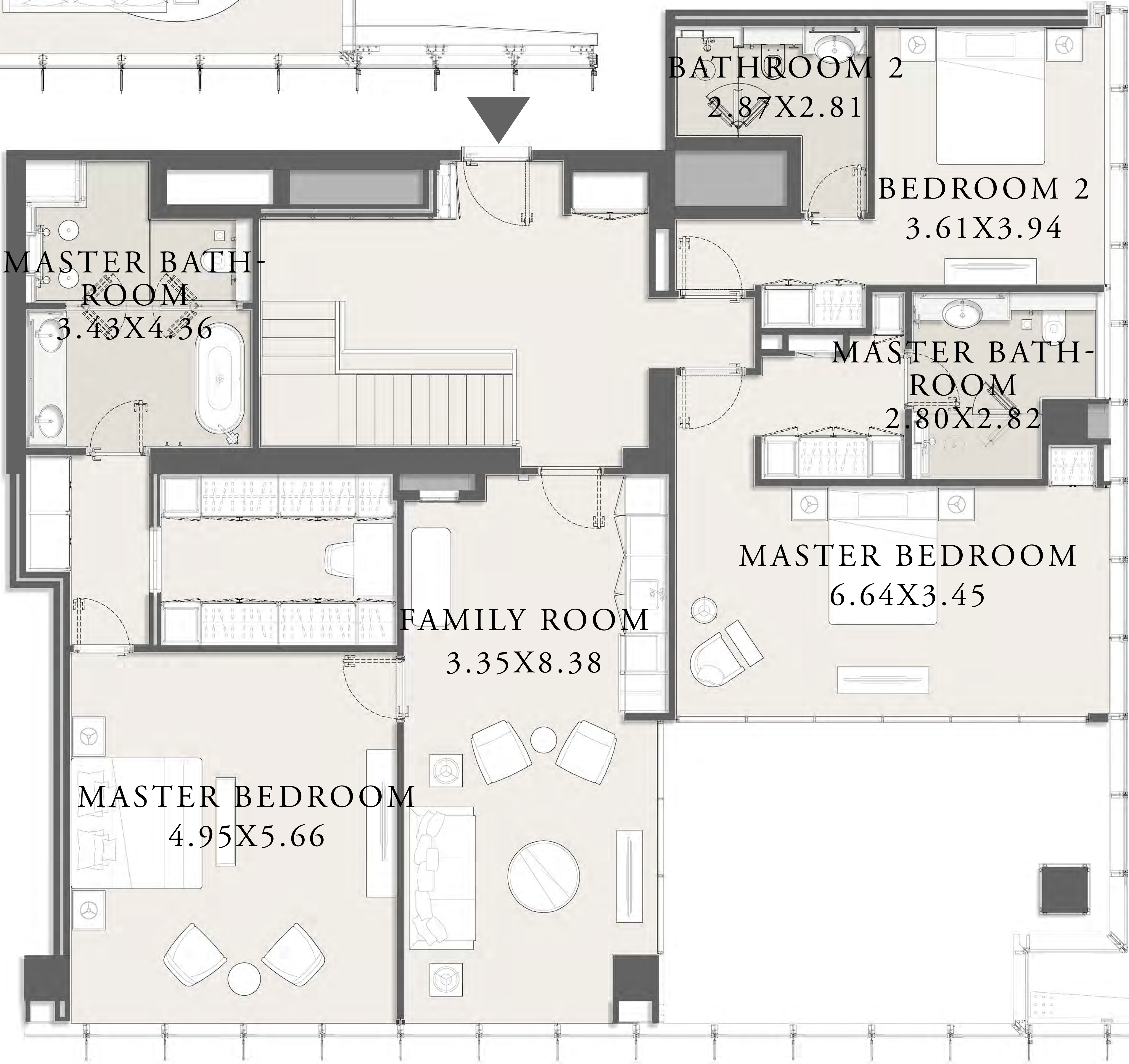
UPPER LEVEL
