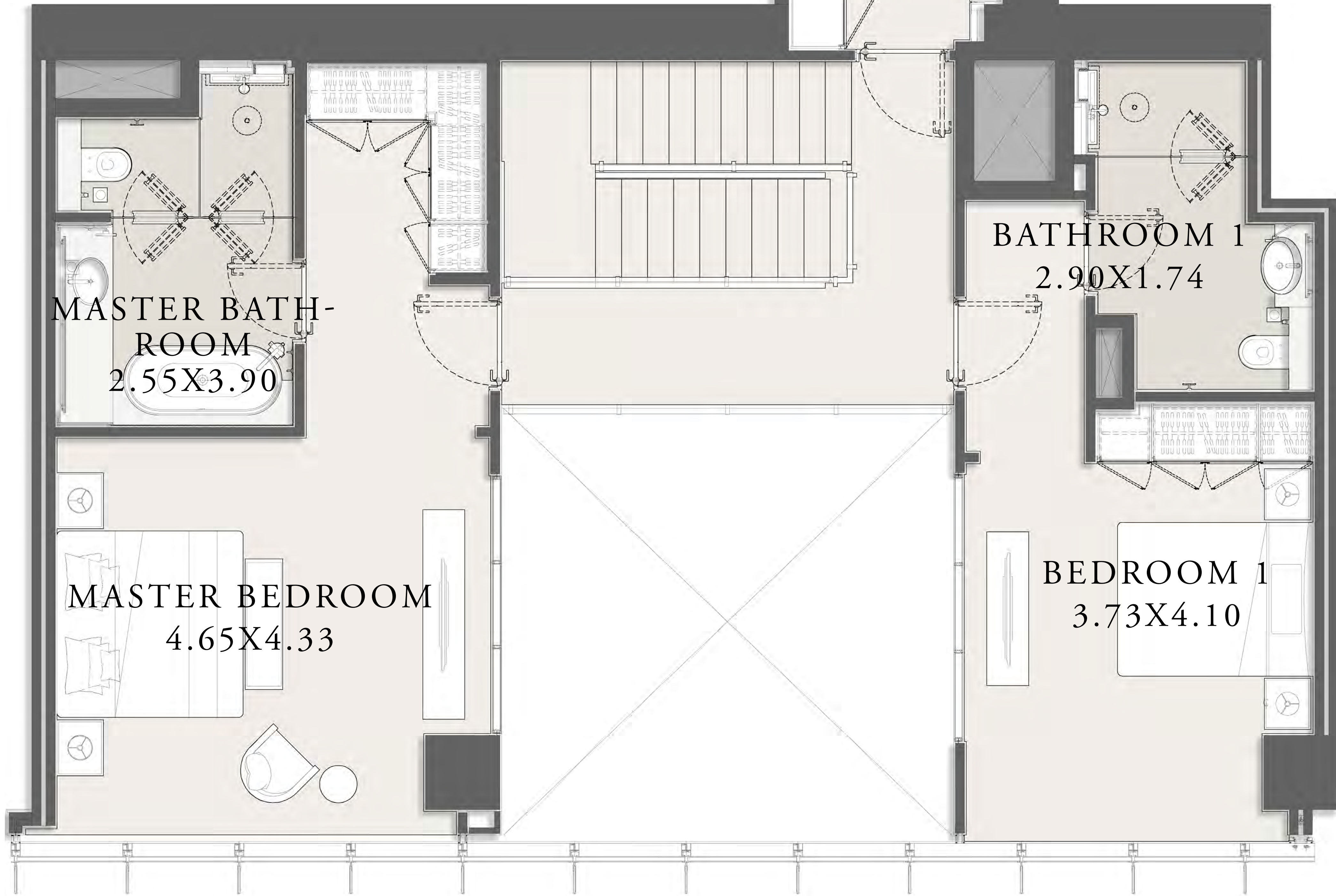
UPPER LEVEL
