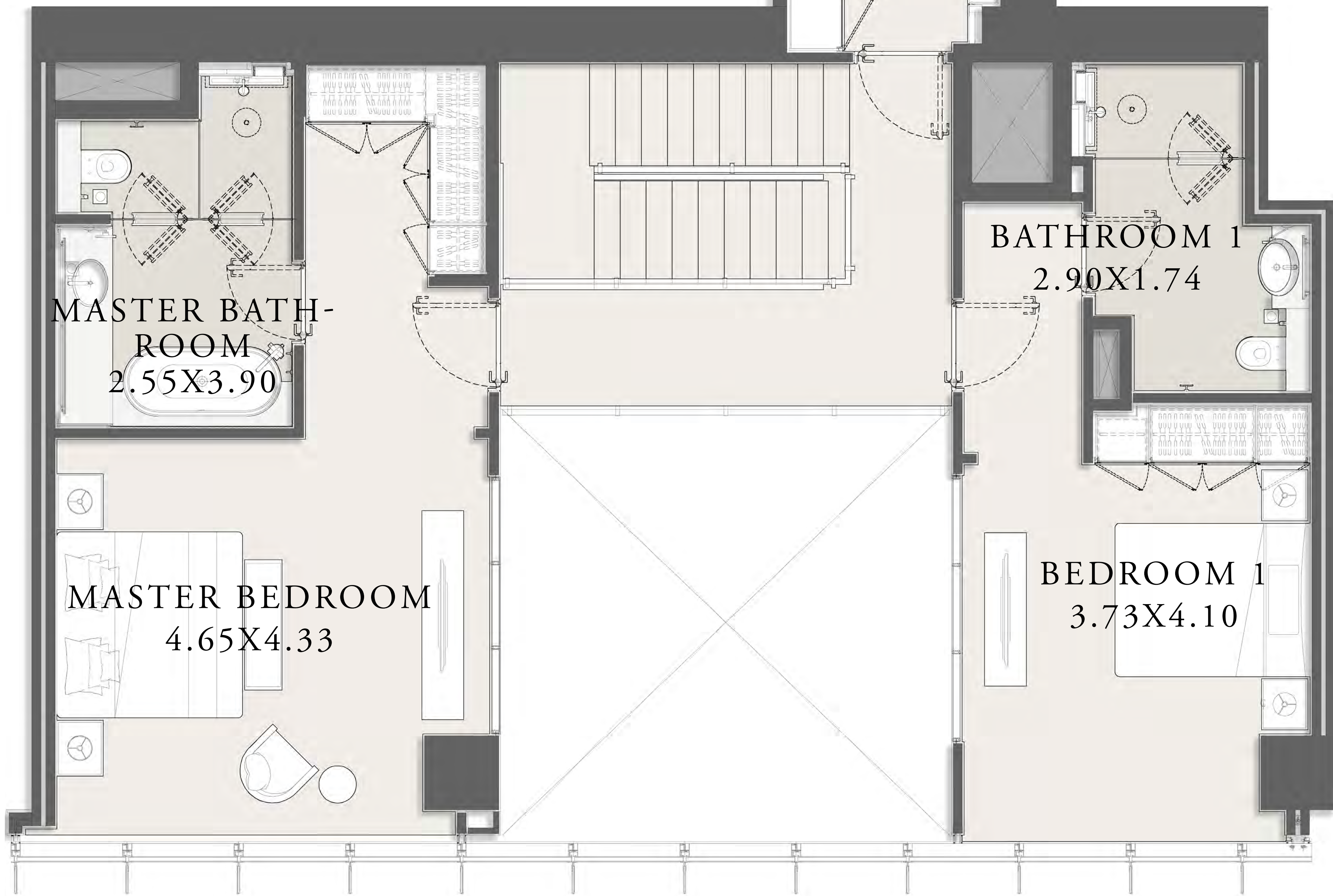
UPPER LEVEL
