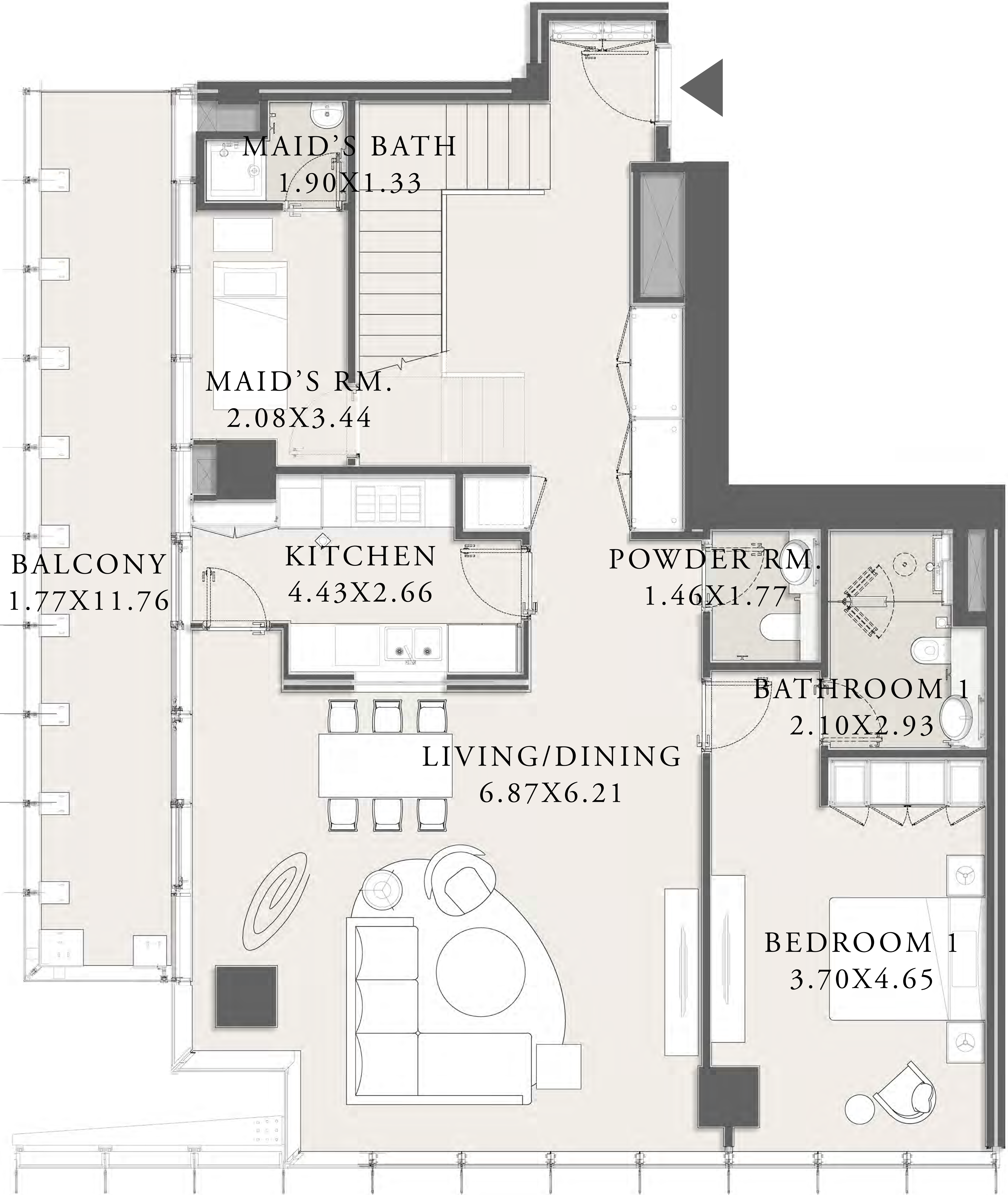
LOWER LEVEL
