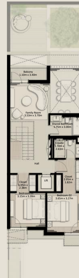
FIRST FLOOR
