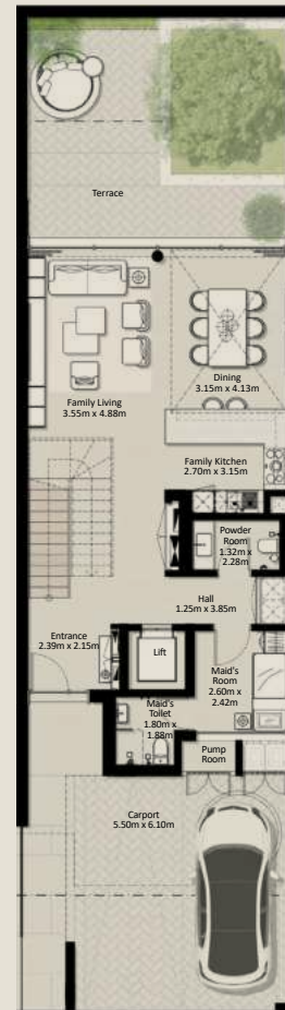
GROUND FLOOR
