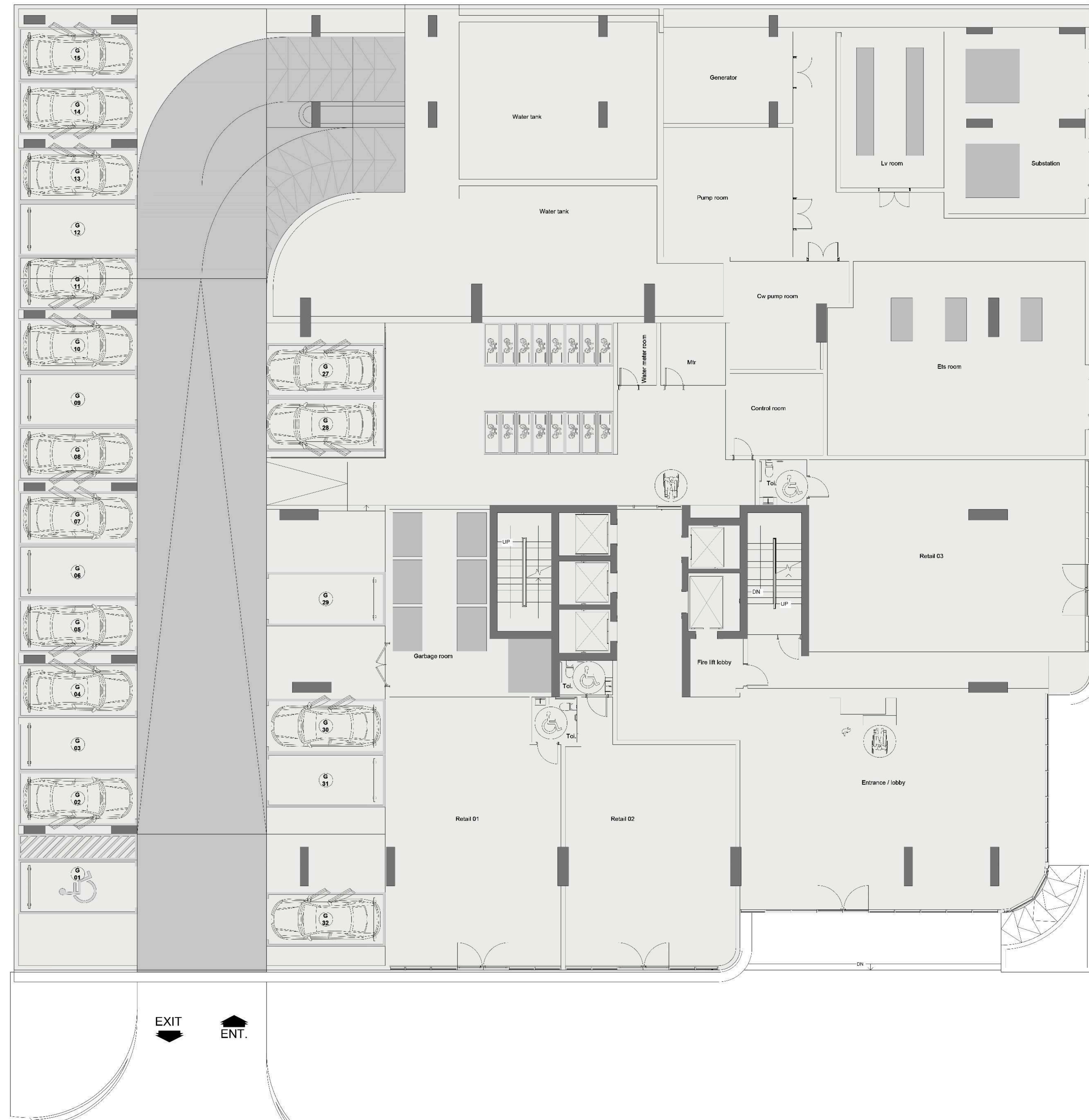
GROUND FLOOR PLAN
