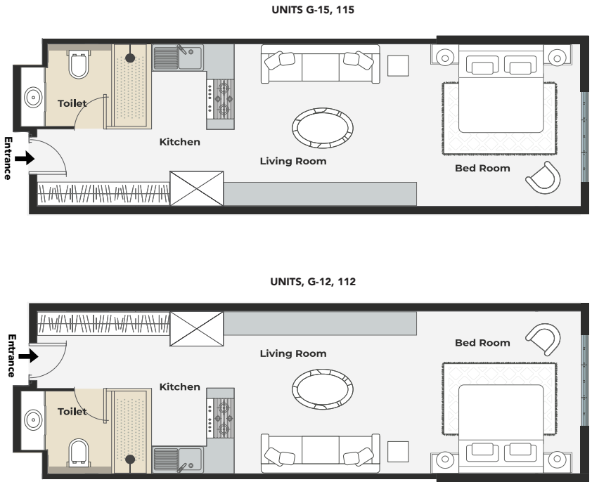
FLOOR PLAN
