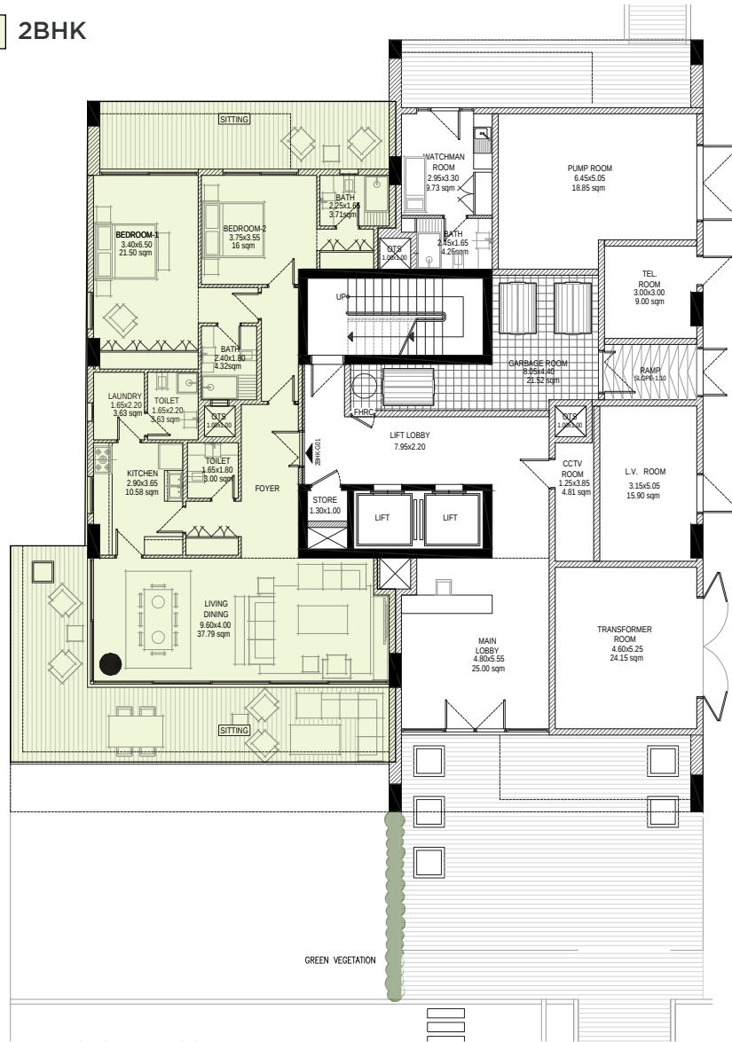
1 GROUND FLOOR PLAN 1:75
