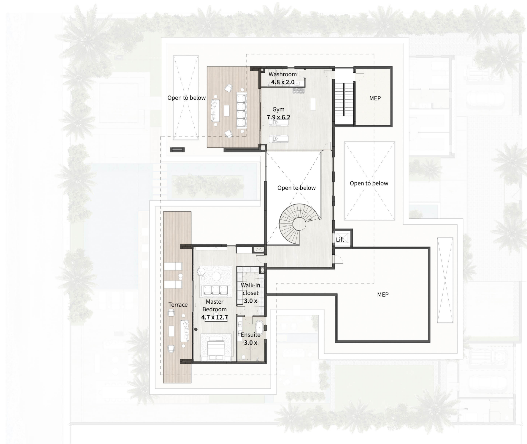
Roof Floor Plan
