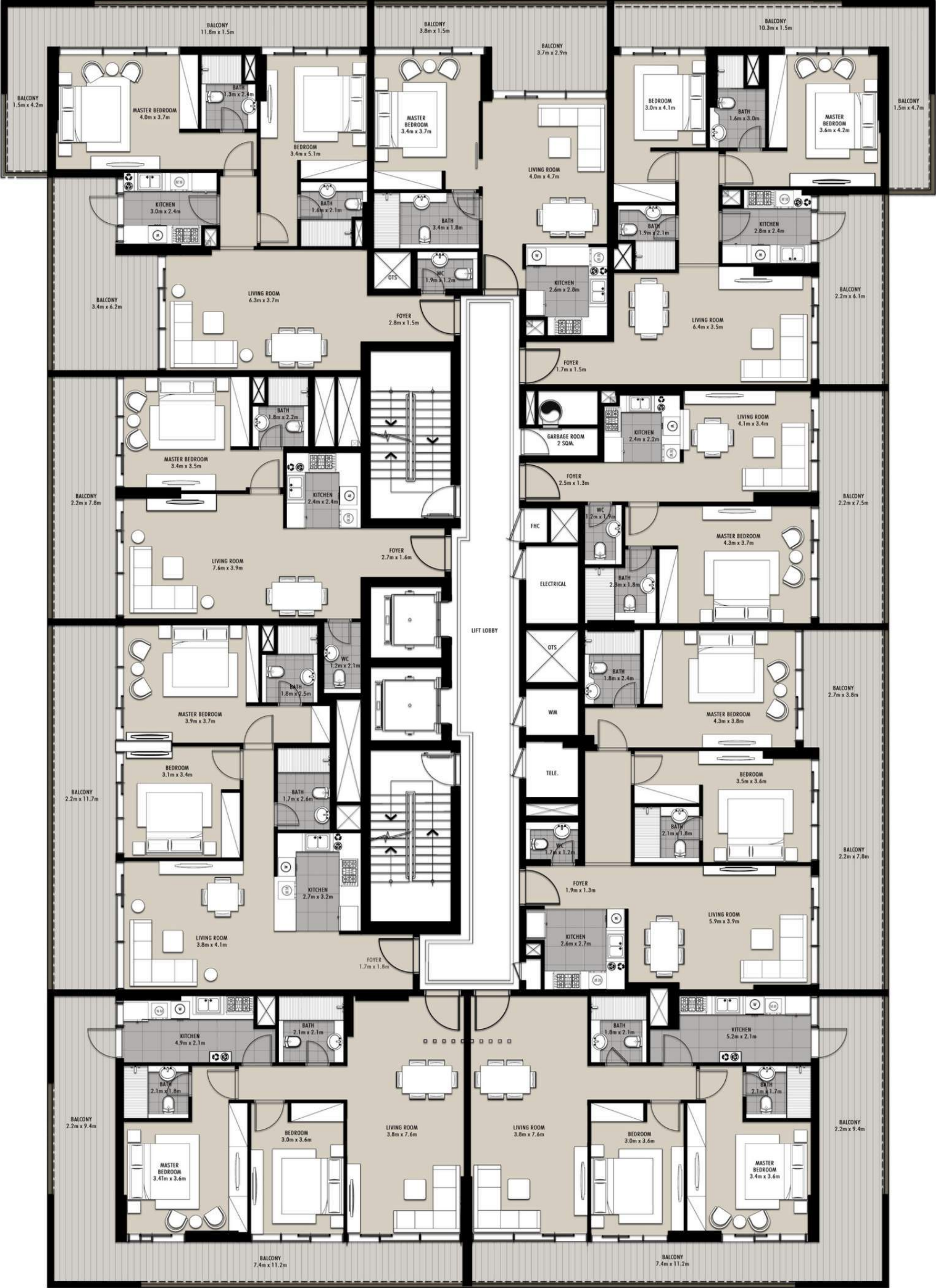
FLOOR PLAN
